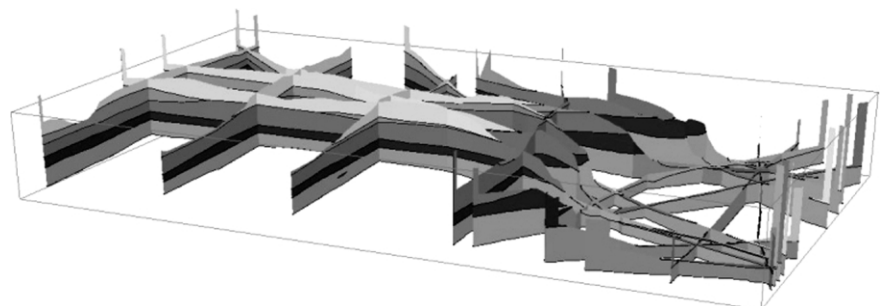
FIGURE 2: 3D visualisation of consistent mesh of cross-sections. Colour coding according to litho-stratigraphy: greyish colours = aeolian sediments and fluvial deposits, black colour = glacial loam and sand, lower most greyish unit = tertiary clay. Vertical exaggeration: 2x
