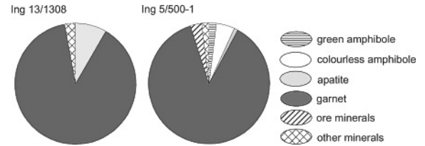
FIGURE 8: Representative heavy mineral data from the base (Ing13/1308) and the top (Ing5/500-1) of the Ingering Formation type section showing the continuous domination of garnet. Heavy minerals (0.0063-0.125 mm fraction) were separated with Tetrabromethane ( \rho = 2.97 \text{ g/cm}^3 ). At least 200 translucent grains were counted.
