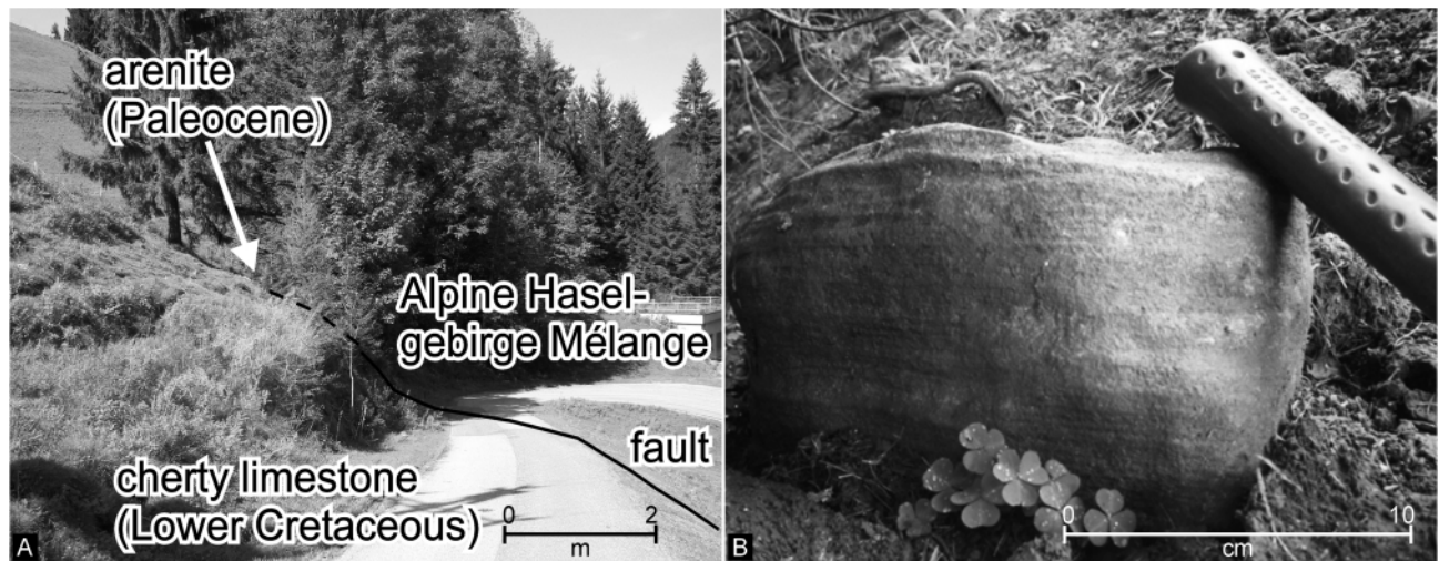
FIGURE 4: A: Geological situation along the road east of Berggasthof Bachrainer. B: Typical calcarenitic rock as typically found at the outcrop. The moderately weathered, subangular sample was dugged out from highly weathered marly country rocks almost completely degraded to soil.
