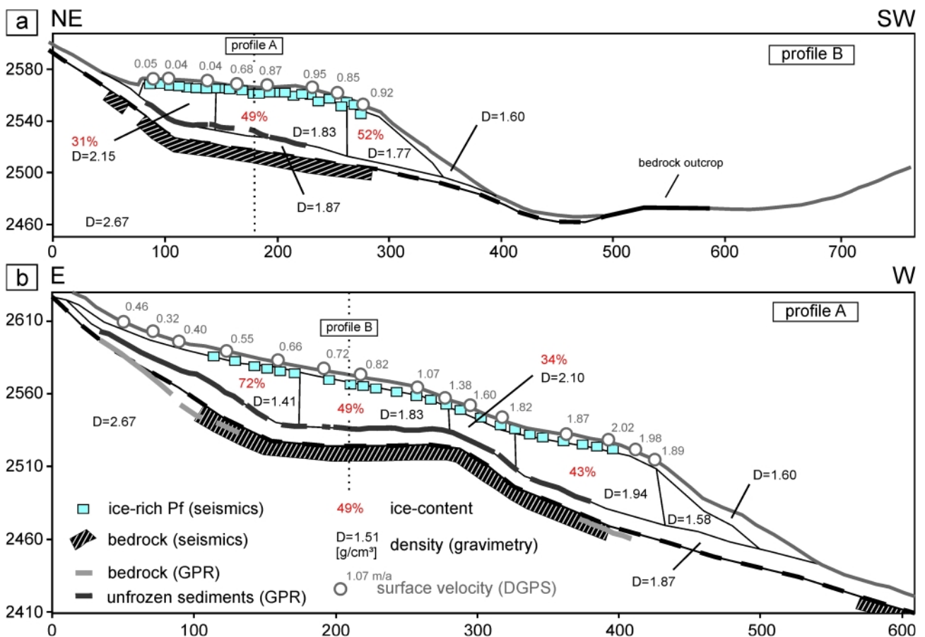
FIGURE 6: The geophysical model of Ölgube rock glacier determined from the integrated methods ground-penetrating radar, seismic refraction, and gravimetry: (a) transverse section along the seismic profile B, (b) longitudinal section along the seismic profile A. The model presents a structural image of the rock glacier with the density distribution and an estimate of the ice content. Mean annual surface velocities during the period 2002 to 2004 are displayed along the flow direction.
