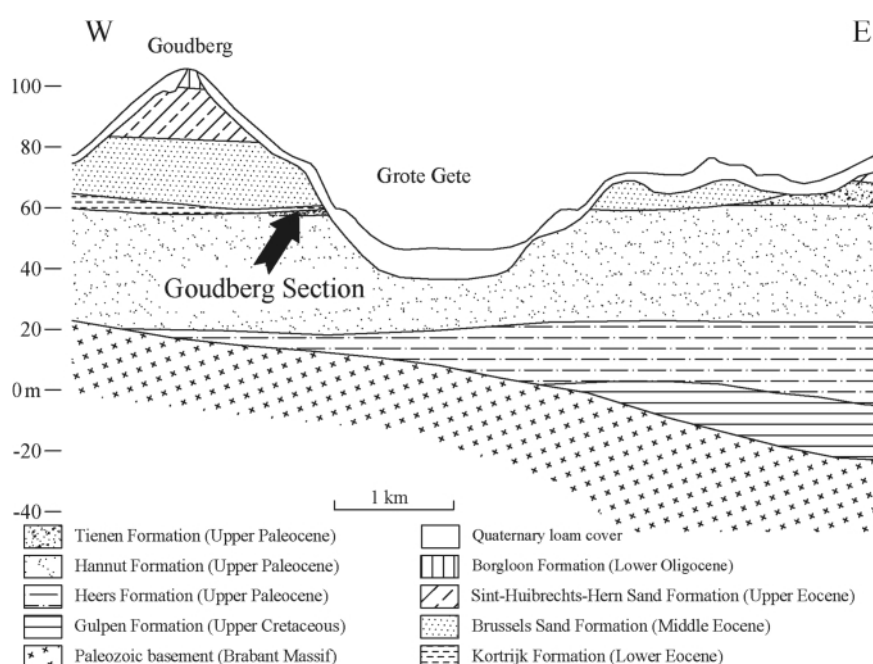
FIGURE 2: Geological section of the Goudberg (modified after Sintubin et al., 2000).
