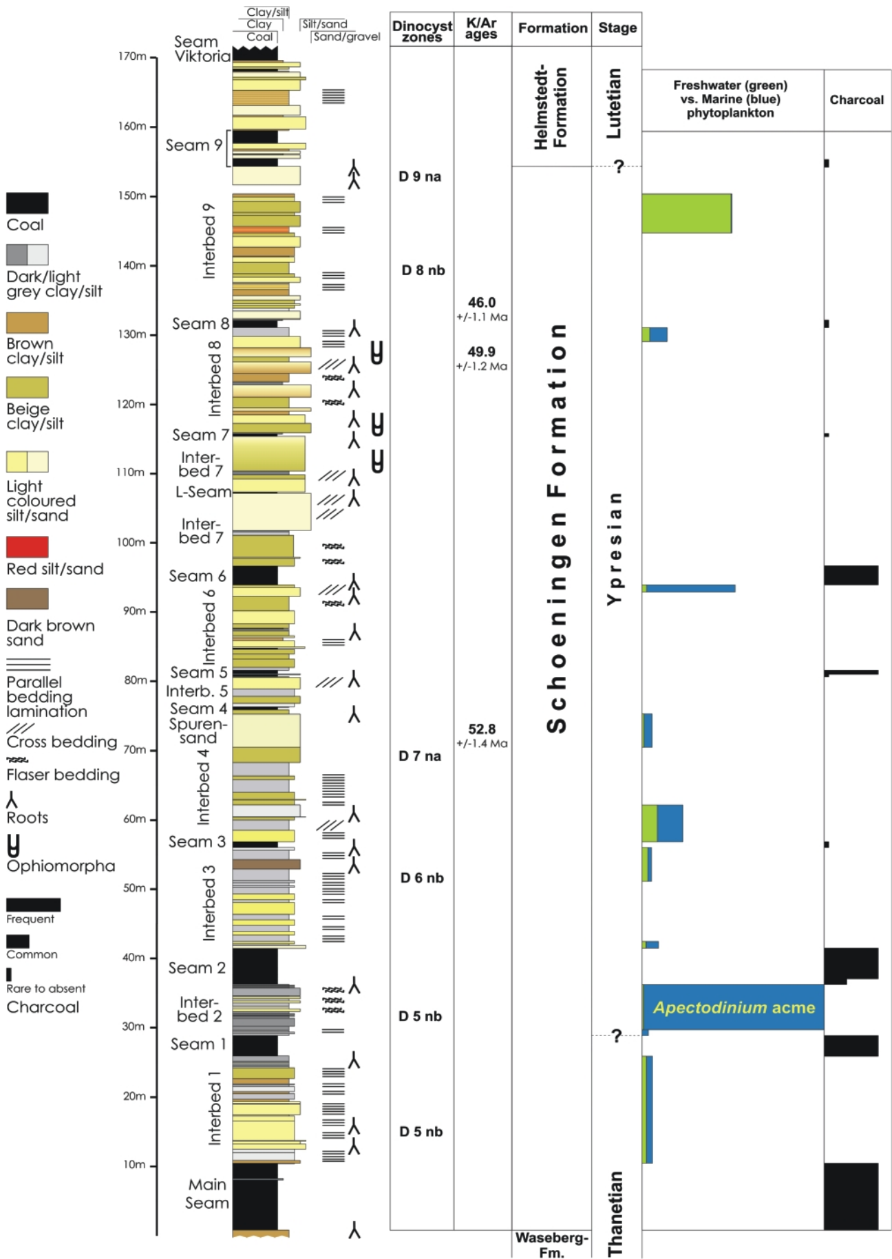
FIGURE 3: Composite section from the central part of the opencast mine Schöningen Süd. Position of scattered data on dinocyst zones and radiometric ages have been transferred from Ahrendt et al. (1995) as shown in Lietzow and Ritzkowski (2005).
