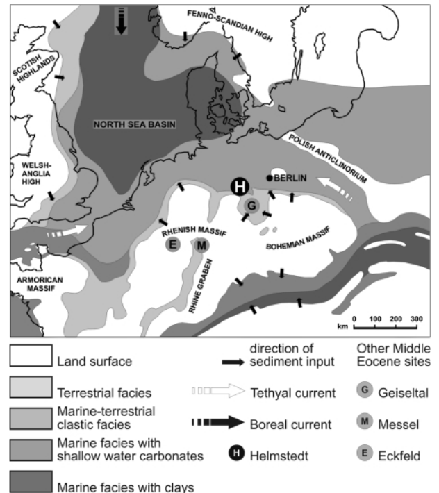
FIGURE 1: Palaeogeographic map of northwestern Europe during the Early Eocene (adapted from Ziegler, 1990) showing the position of the Schöningen section in relation to well-known Middle Eocene fossil sites such as the Geiselst, Messel and Eckfeld.
