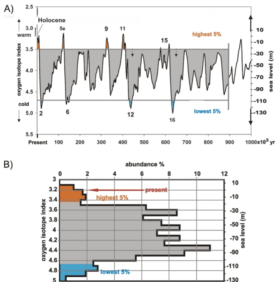
FIGURE 13: Eustatic sea level fluctuations of the past 900 000 yr, reconstructed from oxygen isotope ratios ( \delta^{18}\text{O}/^{16}\text{O} ) of marine calcareous microfossils. (A) Sea-level curve shows that highstands comparable to the Holocene existed only for about 5% of time in the past 900 000 yr. (B) Frequency histogram of sea level curve of (A) indicates that Holocene sea level is high but not absolute top. It had been exceeded during two earlier interglacials, strongly suggesting that there currently exist ice sheets that may collapse and melt relatively quickly upon further warming. (Berger, 2008; modified).
