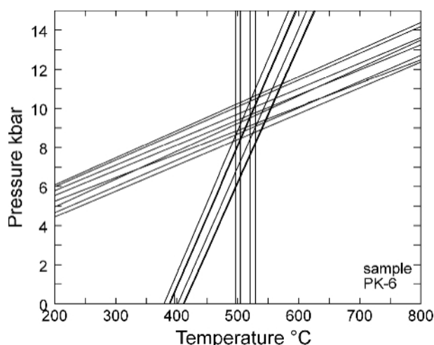
FIGURE 7: P - T estimates of sample PK-6 based on the Fe – Mg exchange reactions between garnet 2 and phengite and garnet 2 and biotite and the net transfer reaction garnet 2 – muscovite – plagioclase 2 – quartz.
