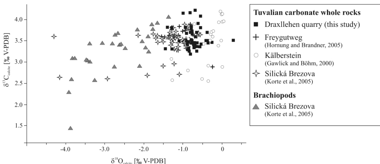
FIGURE 6: \delta^{13}\text{C}_{\text{carb}} / \delta^{18}\text{O}_{\text{carb}} -crossplot of the Draxllehen carbonate rocks and other investigated Tuvanian Hallstatt Limestone sites.
