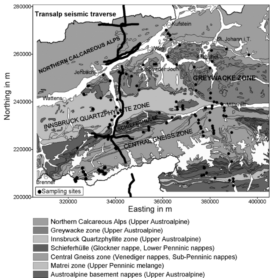
FIGURE 3: Geological sketch map (modified from "Metallogenetische Karte von Österreich 1 : 500000", Ebner et al., 1997) of the investigated area with the locations of sampling sites (black dots). Tectonic units according to Schmid et al. (2004) and Frisch (1979).
