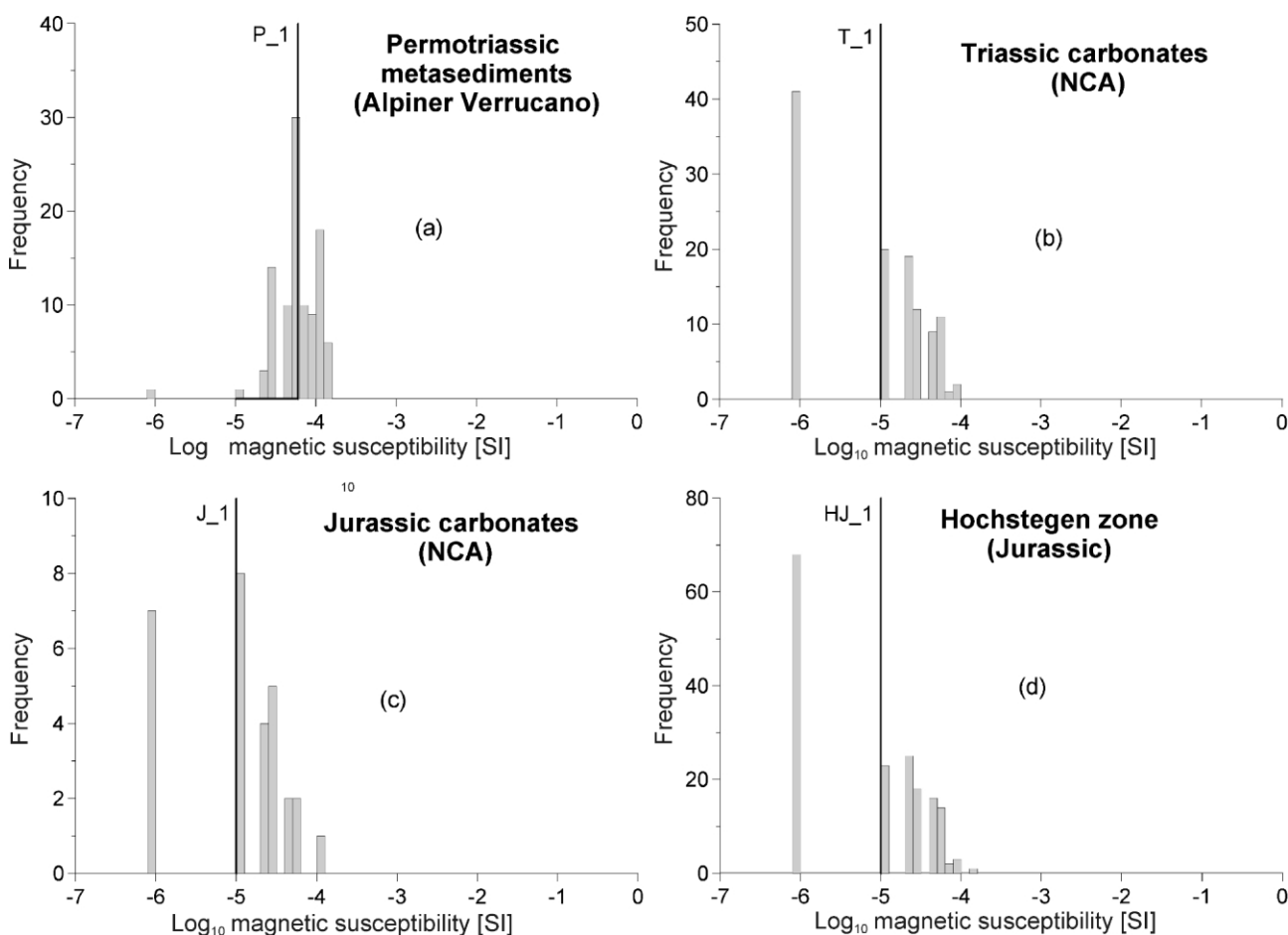
FIGURE 4: Distribution of the magnetic susceptibility of Permian Triassic, Triassic and Jurassic rocks. (a) siliciclastic "Alpine Verrucano", NCA, (b) Triassic carbonates of the NCA, calcitic and dolomitic marbles of the Seidlwinkeltrias and dolomitic marbles of the Krimmler Triassic rocks (c) Jurassic (mainly Liassic) carbonates of the NCA, (d) Jurassic Hochstegen marble of the Venediger nappe (Mesozoic cover of the Sub-Penninic Ahorn core).
